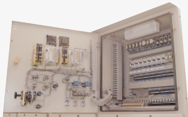
LV Compartment
