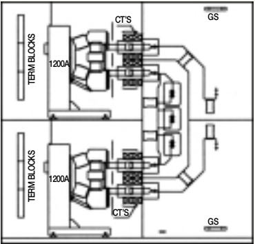
Breaker / Breaker (Top and Bottom Entry)
