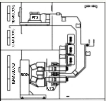
Auxiliary / Breaker (Top Entry) *4.76 kV Only
