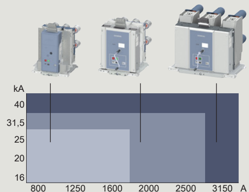
SION vacuum circuit-breaker 3AE5 for 17.5 kV
