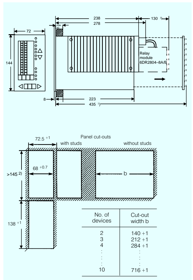
Fig. 16/16 SIPART DR22 controller and panel cut-outs, dimensions
