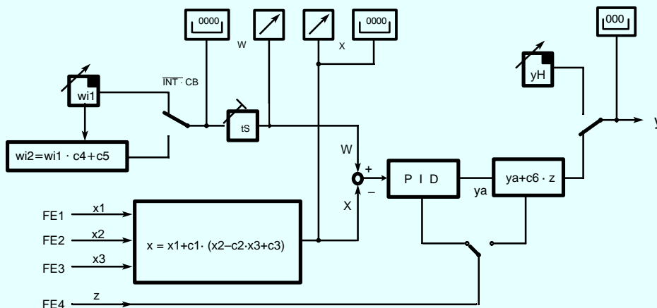
Fig. 6/5 Fixed setpoint controller with two dependent setpoints, function diagram
