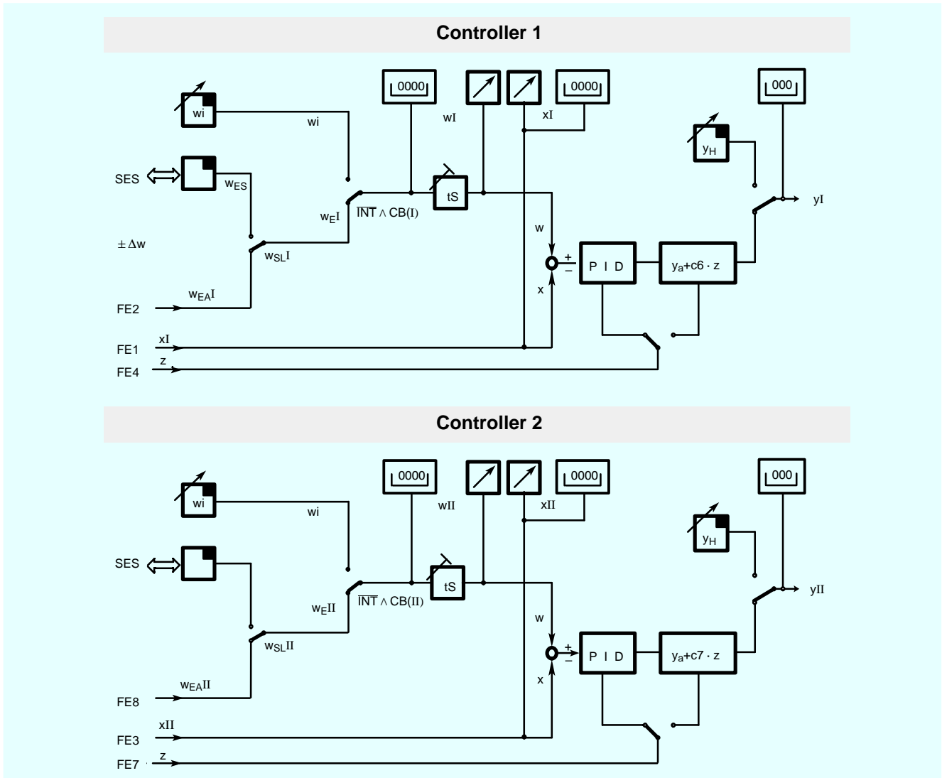
Fig. 6/12 Dual loop controller
