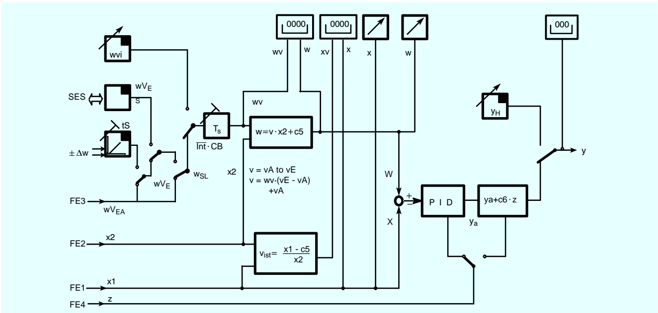
Fig. 6/8 Fixed or controlled ratio controller, function diagram
