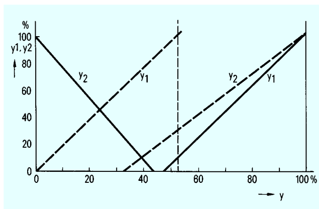
Fig. 6/13 Possibilities of split-range mode
