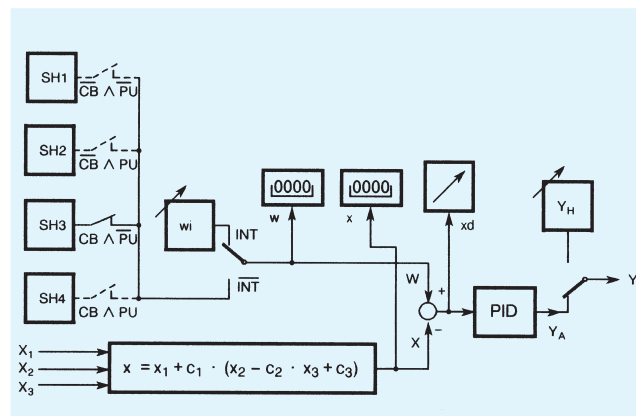
Fig. 3/4 Fixed setpoint controller with 5 independent setpoints as one, two or three-component controller
