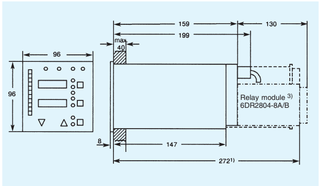
Fig. 3/13 SIPART DR19 controller, dimensions in mm
